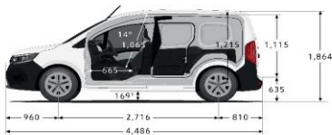
Dimensions (mm)
